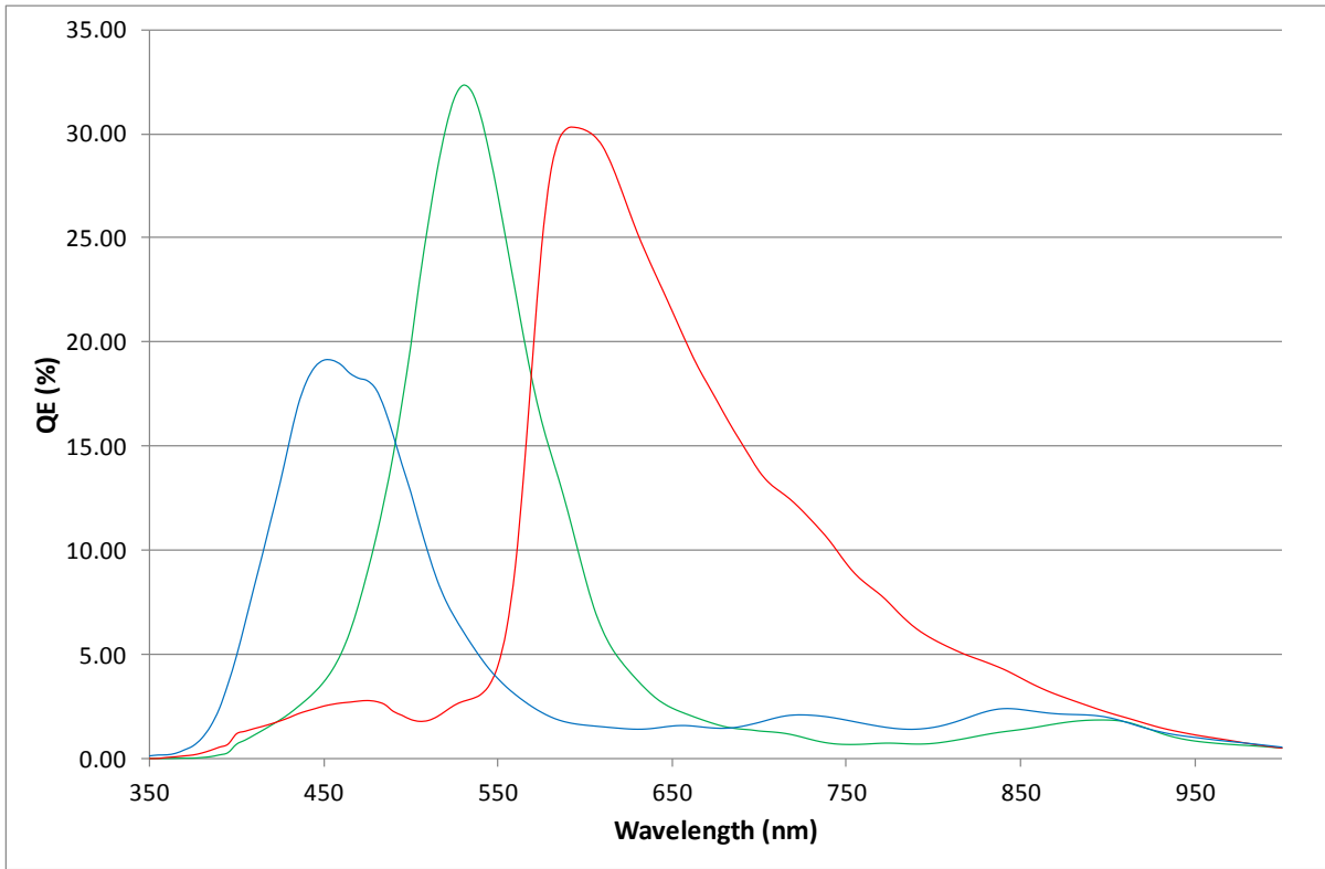
Figure 7: Typical Quantum Efficiency (QE) versus wavelength
