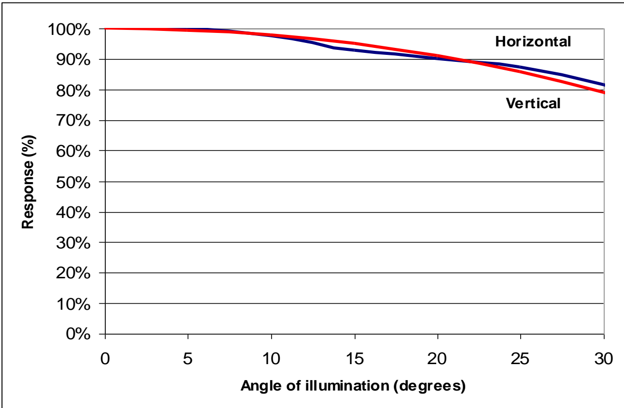
Figure 8: Angular response versus angle of illumination
