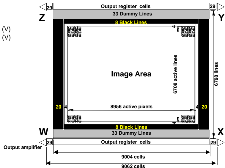
Figure 1: Device Structure
